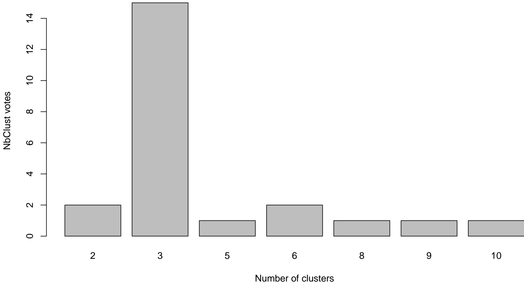
NbClust: Votes per k (ward.D2)
