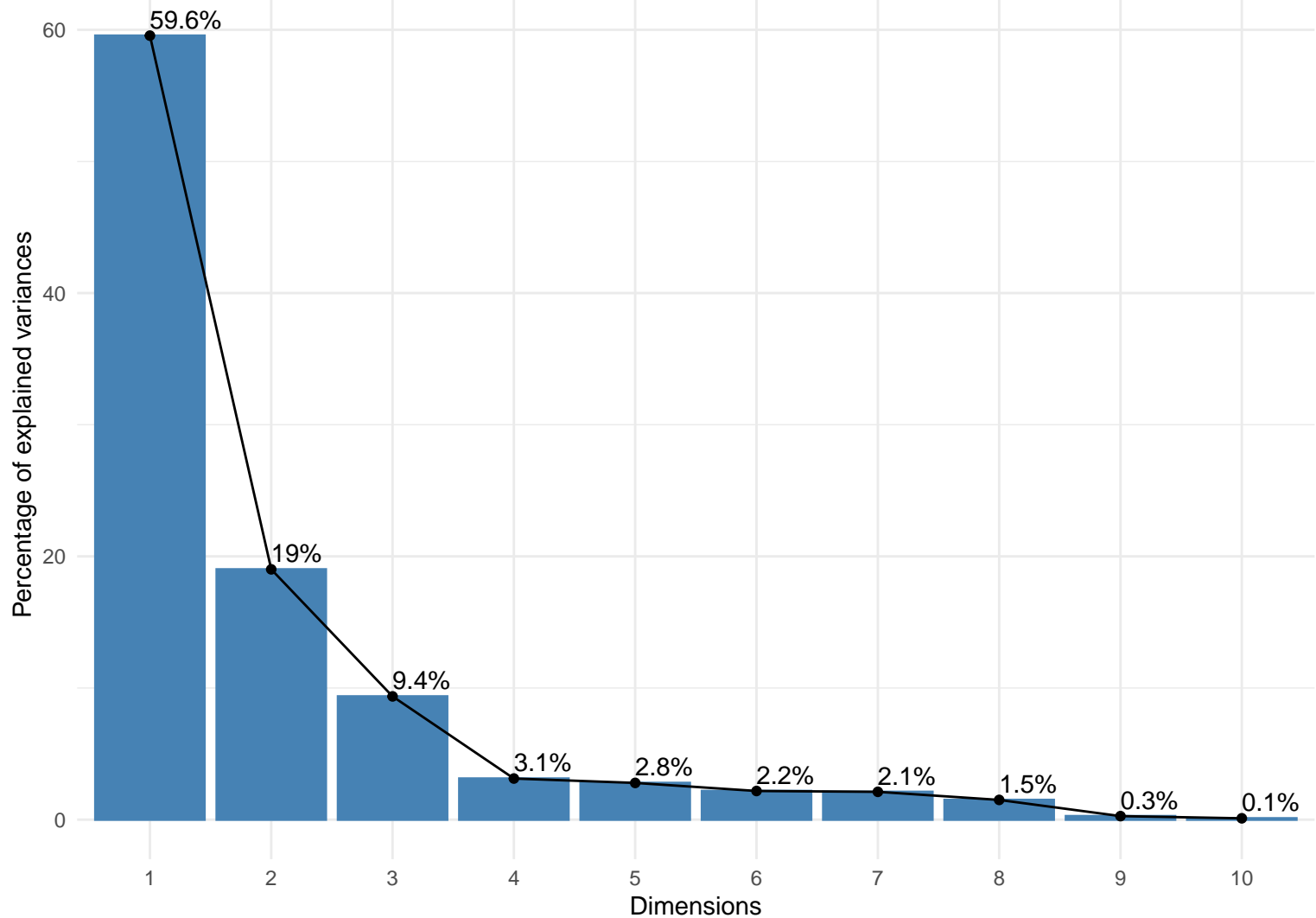
PCA Scree Plot – Variance Explained by Each Component
