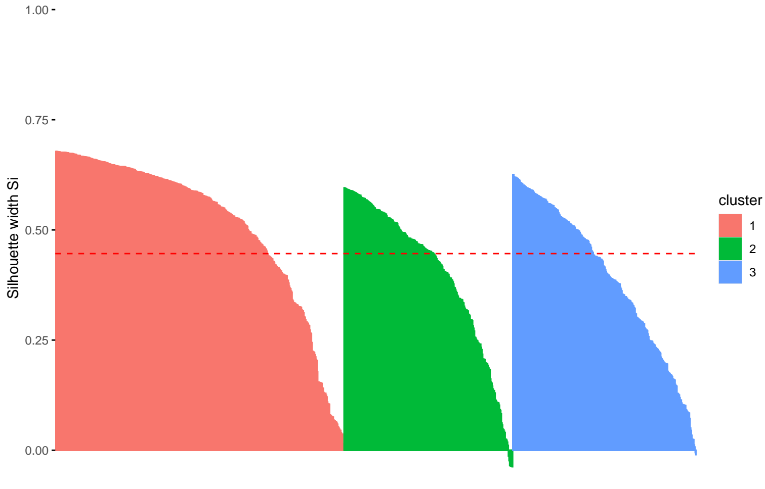
Clusters silhouette plot Average silhouette width: 0.45
