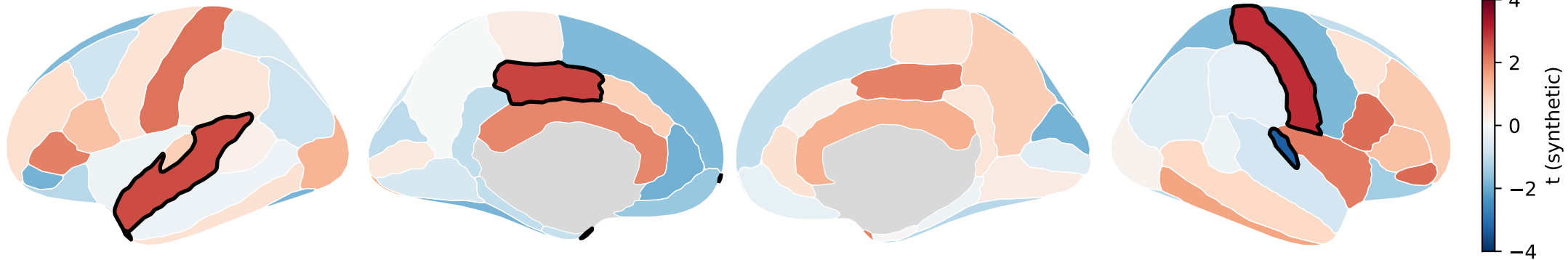
Cortical t-map — black outline: |t| > 2.3
