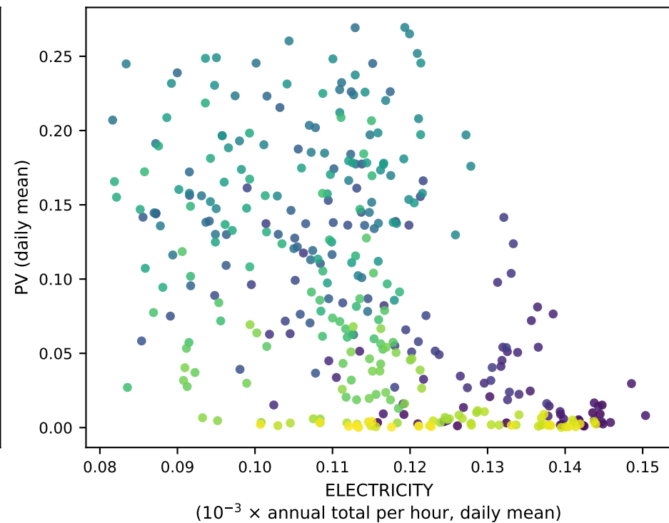
Finland daily-mean co-variation (2017, UTC) Electricity vs PV r = -0.506
