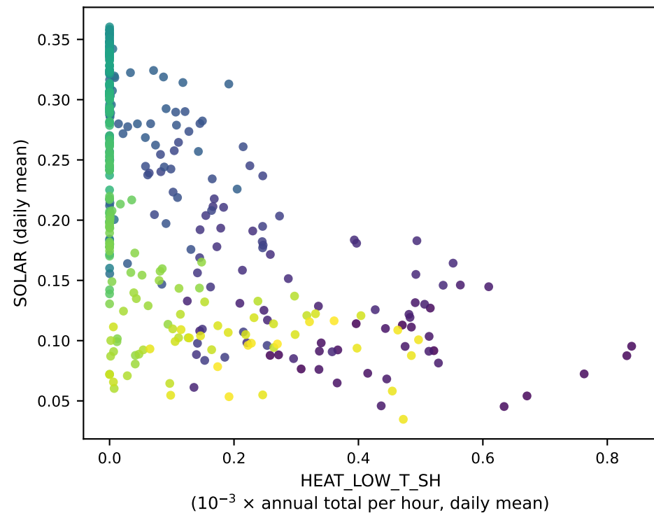
Heating vs solar r = -0.614
