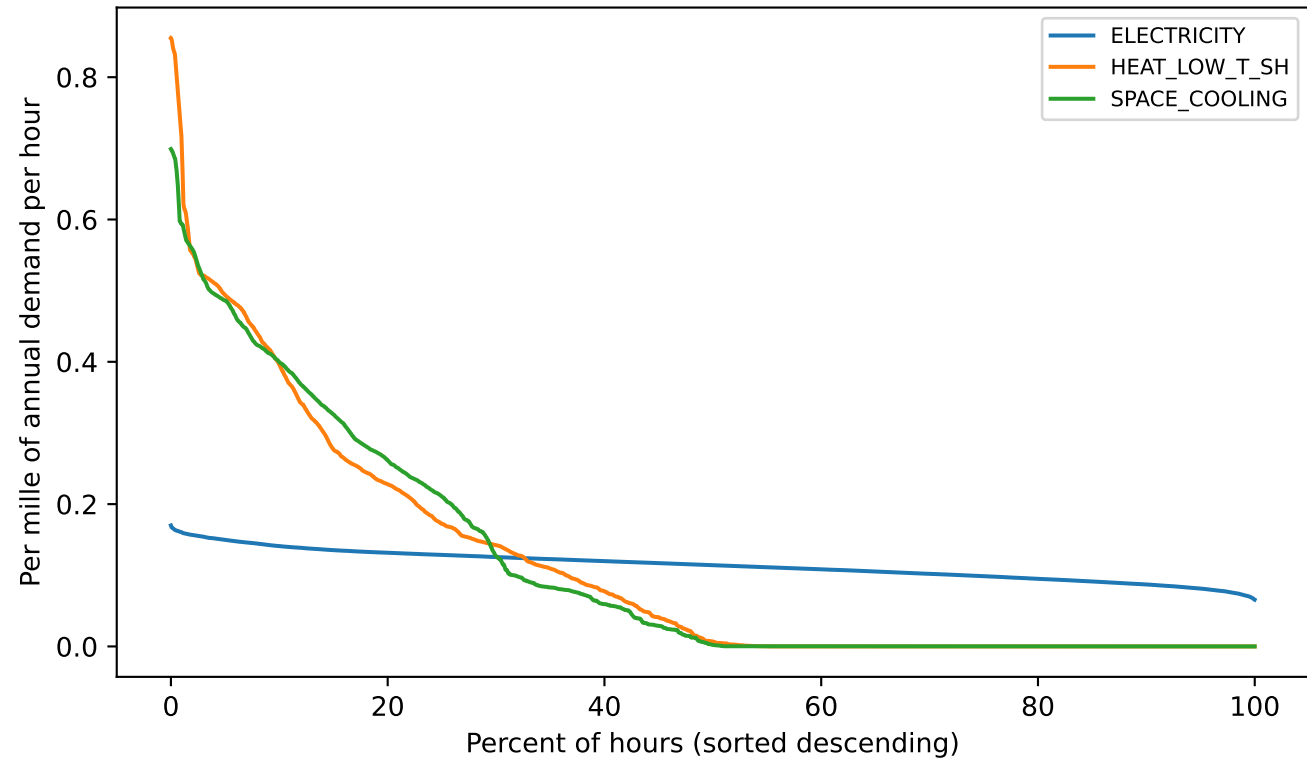
Finland demand duration curves (2017, UTC)
