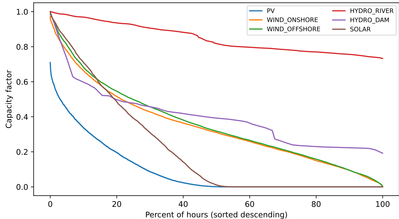
Finland renewable duration curves (2017, UTC)
