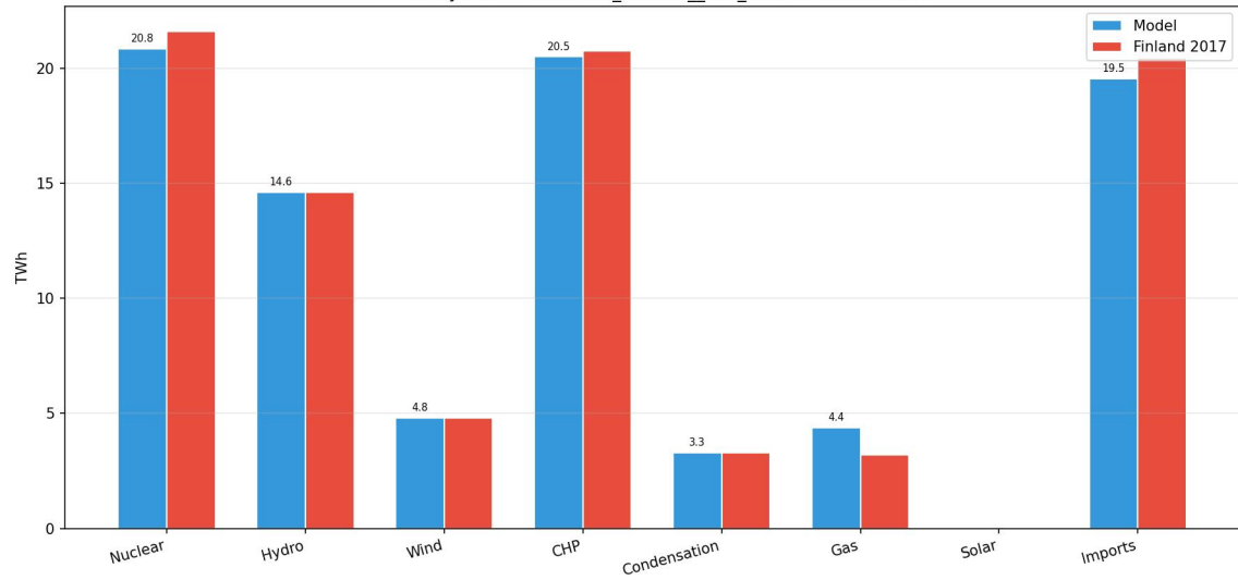
Electricity Mix — 20260323_173930__v37_solar vs Finland 2017
