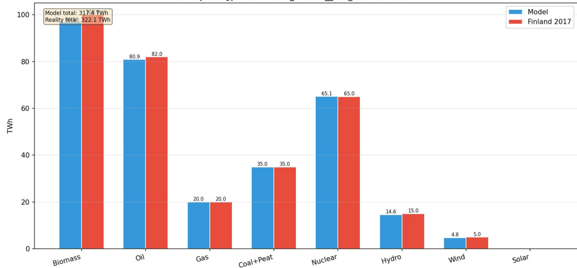
Primary Energy — 20260323_173930_v37_solar vs Finland 2017
