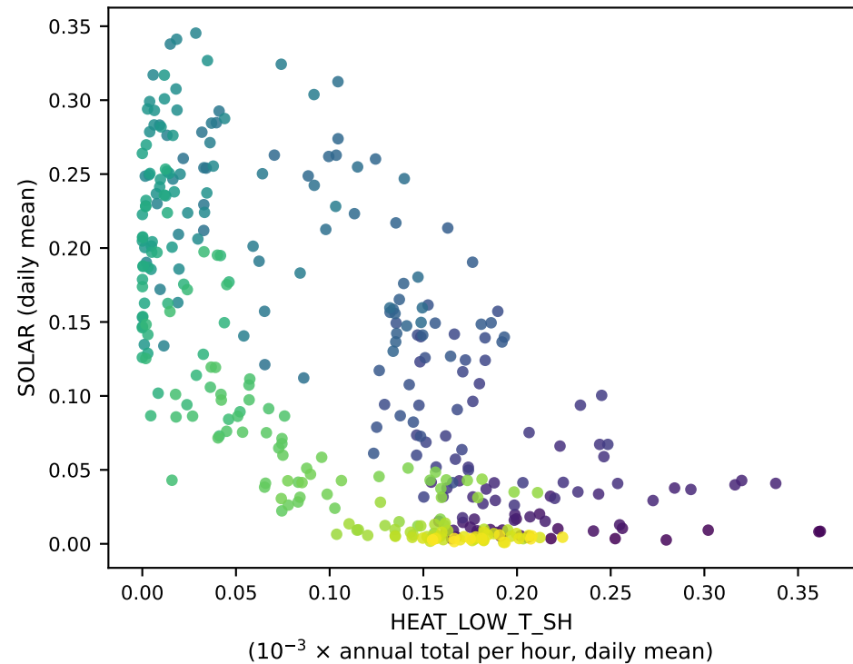
Heating vs solar r = -0.693
