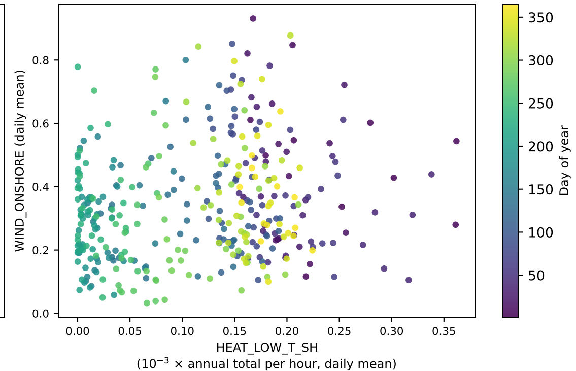
Heating vs wind (onshore) r = 0.175
