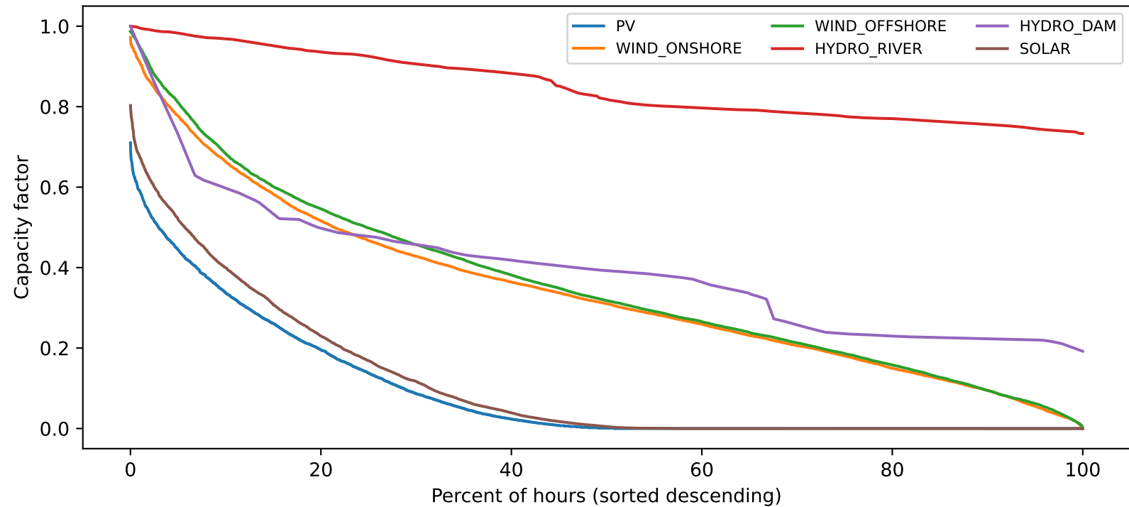
Finland renewables duration curves (2017, UTC)
