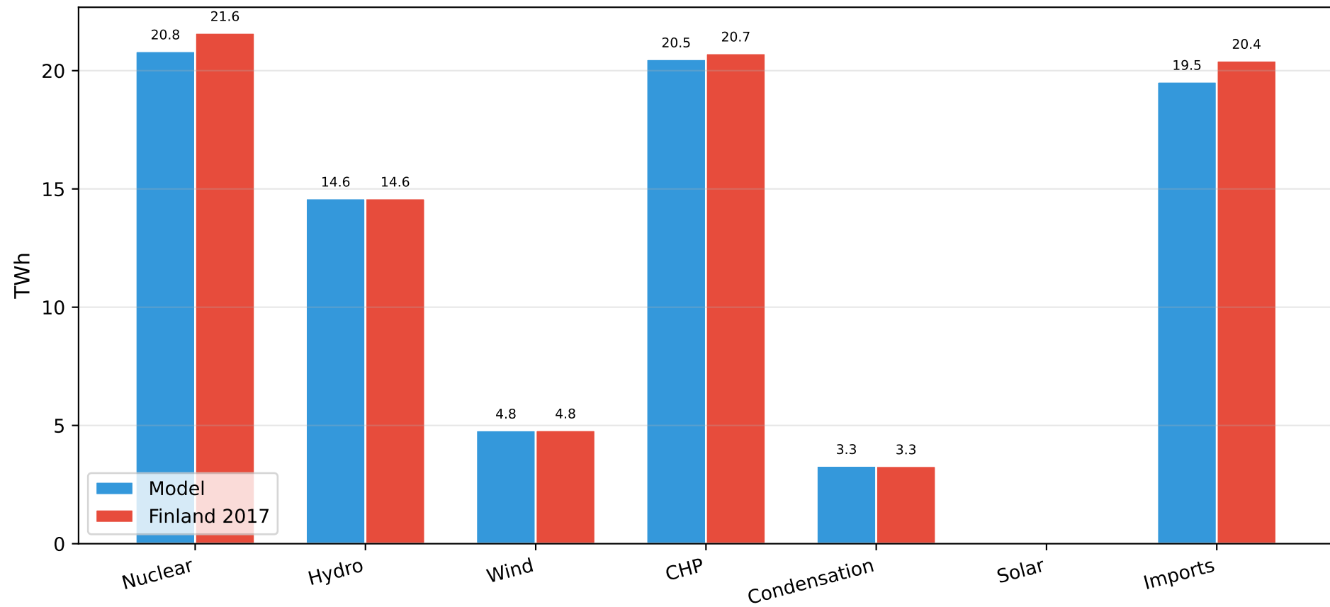
Electricity generation by technology — model vs. Finland 2017 statistics
