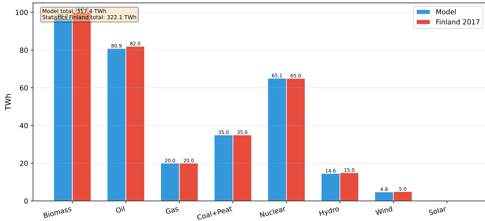
Primary energy supply by carrier — model vs. Finland 2017 statistics
