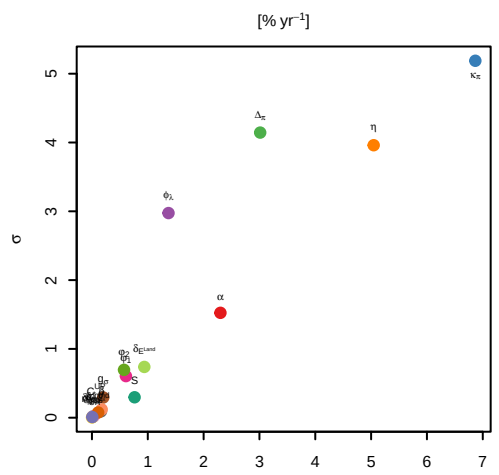
Inflation (avg. 2050–2100)
