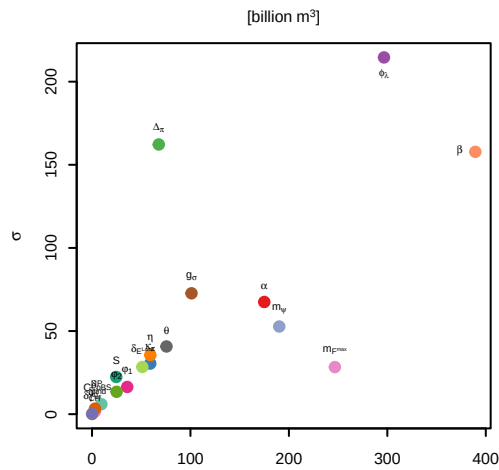
Cumulative emissions (2020–2100)
