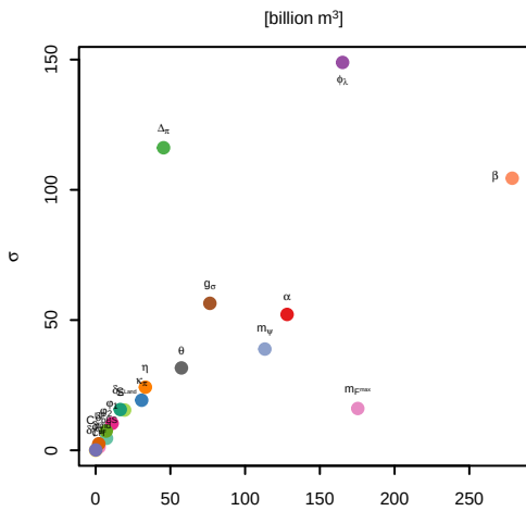
Emissions (2100)
