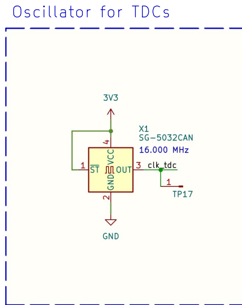
Abbildung 16: Oscillator for TDCs
