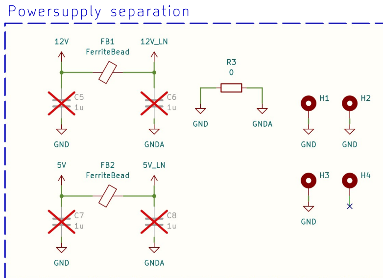
Abbildung 17: Power Supply Separation
