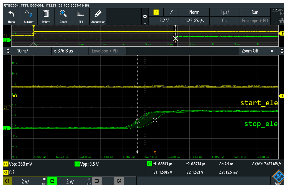
Abbildung 29: GPIO Toggle with HAL - DSO (Zoom)
