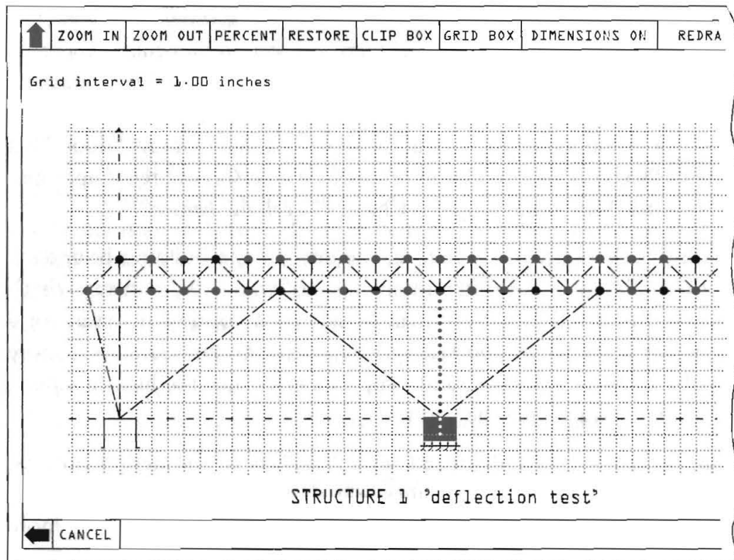
Figure 9.2. Computer Simulation of Structures. Students could enter a proposed design of a structure into the Growltiger program to simulate the structure's behavior under different load conditions. Growltiger was used by students to explore the space of possible bridge designs, and to find surprises that could lead to major shifts in their understanding of their designs. (From Shahaf Gal, "Building Bridges: Design, Learning, and the Role of Computing," 1991 qualifying paper for Harvard Graduate School of Education. Reprinted with permission of S. Gal.)
