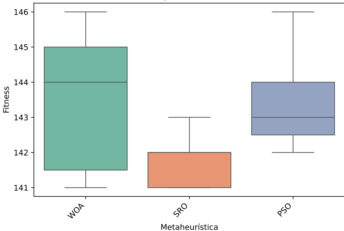
Boxplot Fitness scp61 - V3-STD
