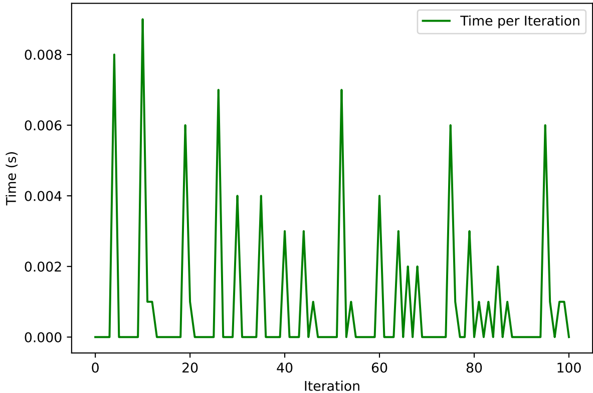
Time per Iteration PSO F4 - Run 30
