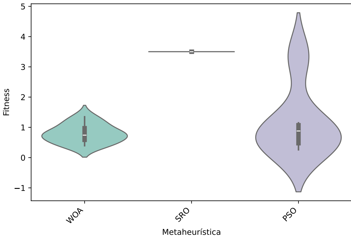
Violinplot Fitness F6
