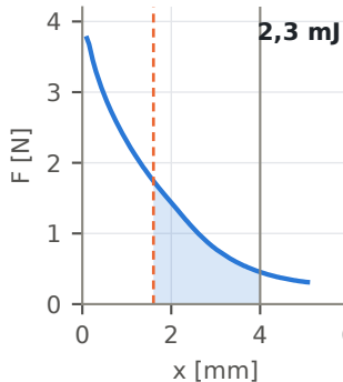
Ledex B12P 13 W (10% ED)
