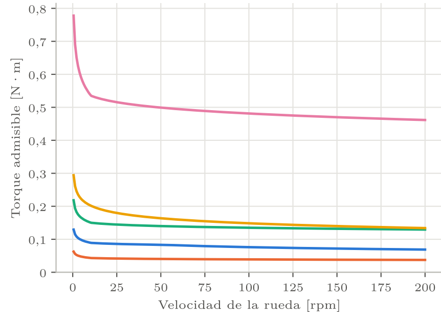
Torque normal
