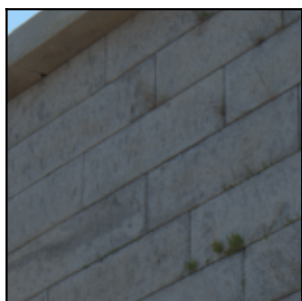
enhance
