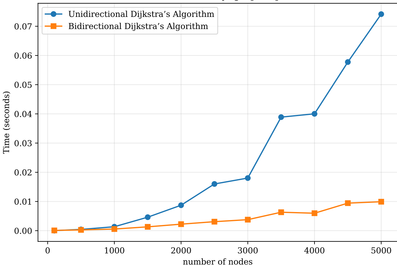
Runtime on Erdős-Rényi graphs ( p = 0.020 )
