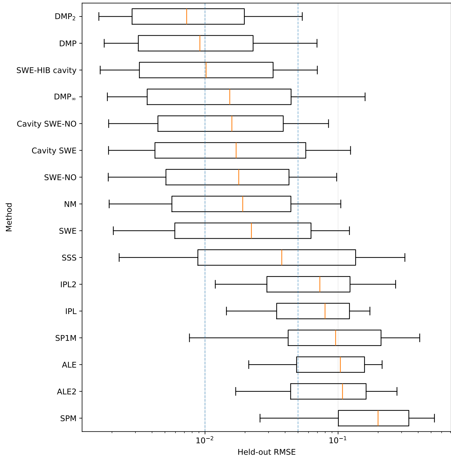
Real-world datasets: held-out RMSE
