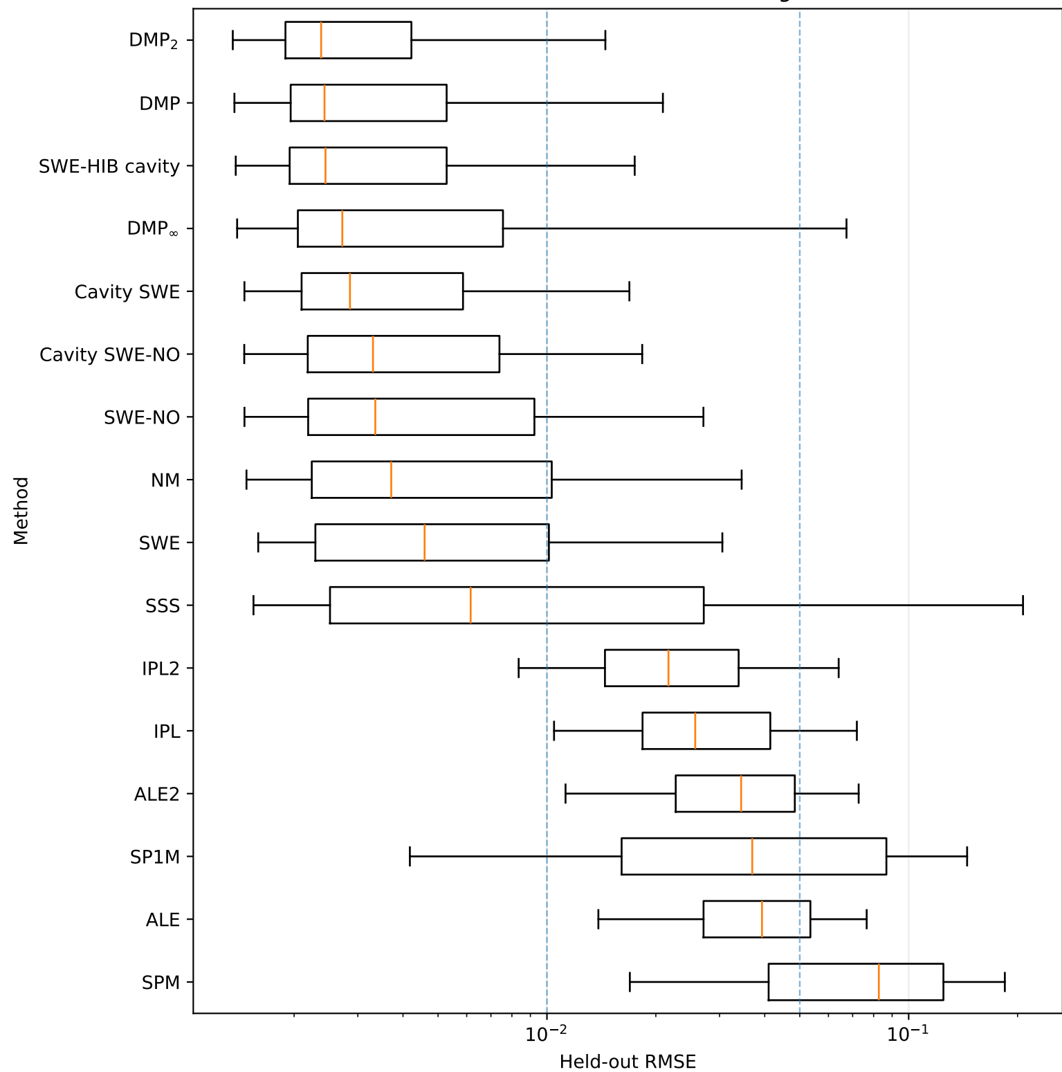
Real-world datasets: held-out RMSE, g^* = 0.10
