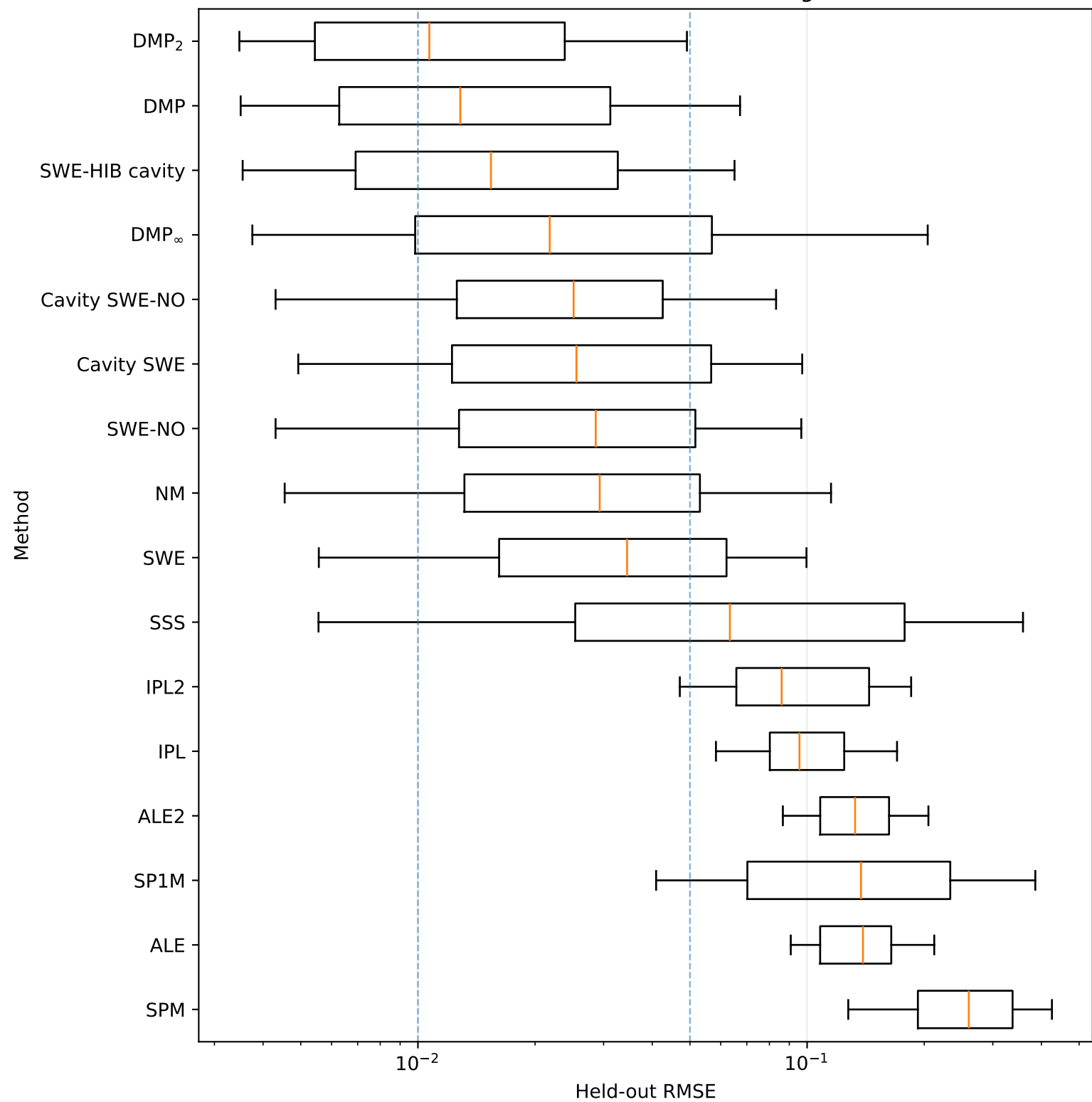
Real-world datasets: held-out RMSE, g^* = 0.35
