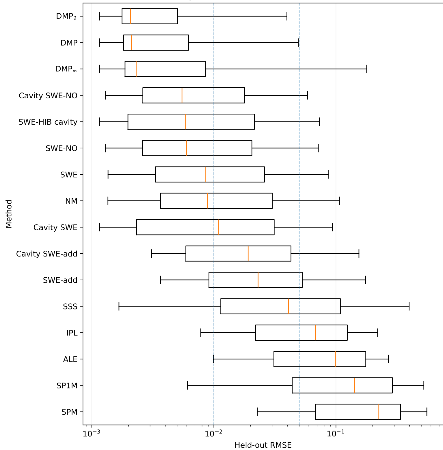
Synthetic datasets: held-out RMSE
