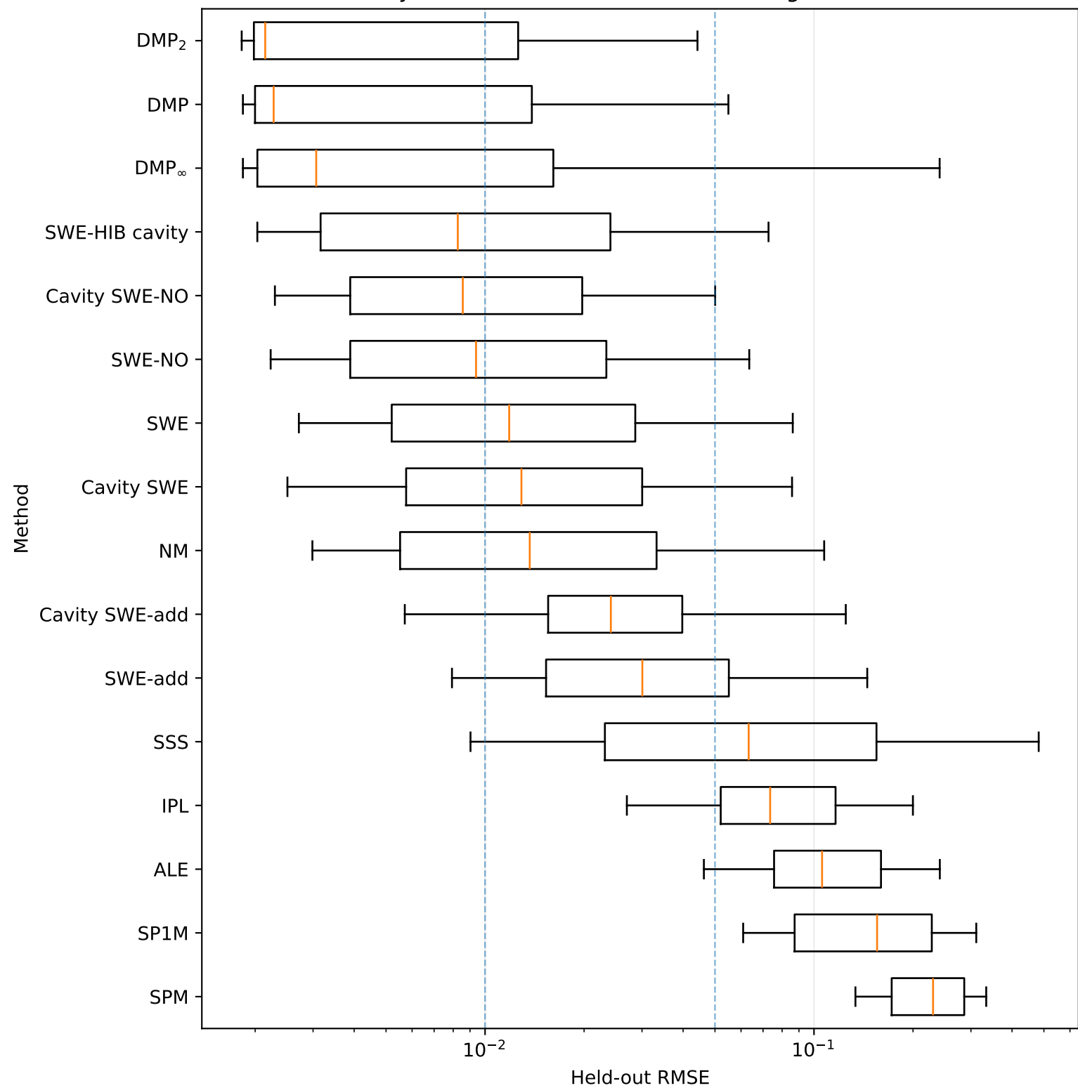
Synthetic datasets: held-out RMSE, g^* = 0.35
