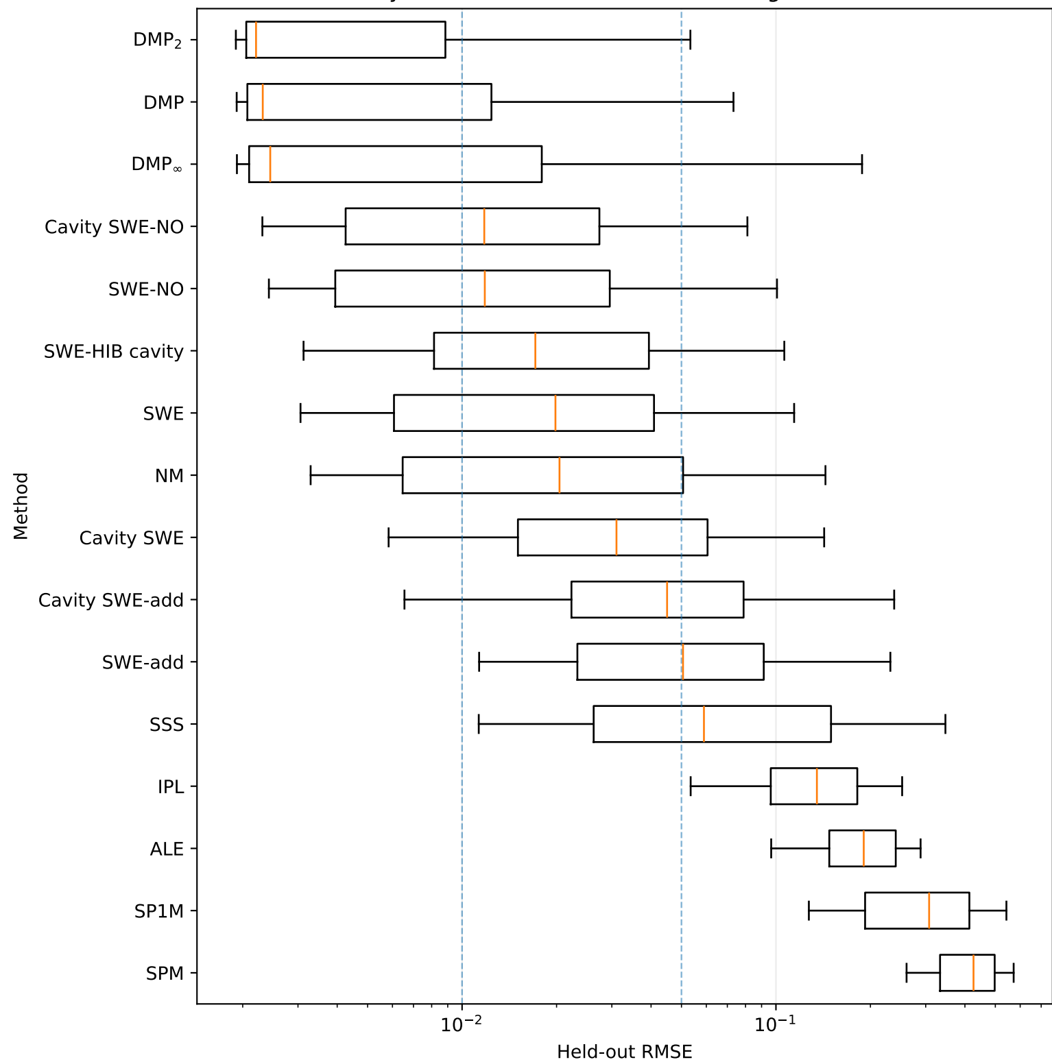
Synthetic datasets: held-out RMSE, g^* = 0.60
