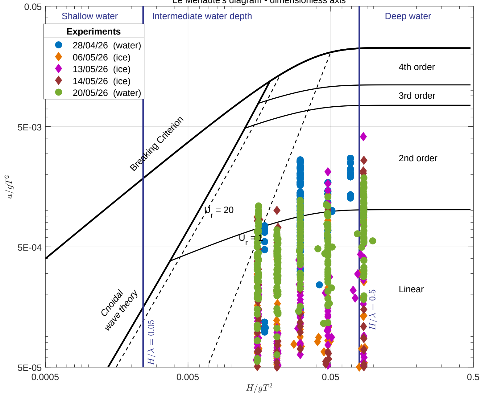
Le Mehaute's diagram - dimensionless axis
