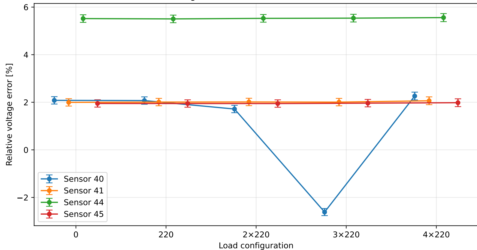
Voltage calibration of INA226 sensors
