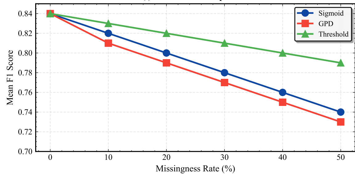
(f) Mechanism Comparison
