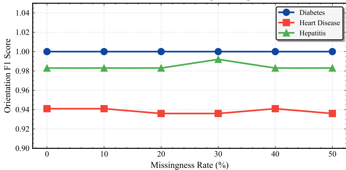
(c) Orientation F1 (Compelled Edges)
