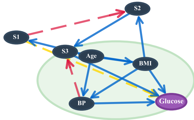
30% missing, F1=0.86
