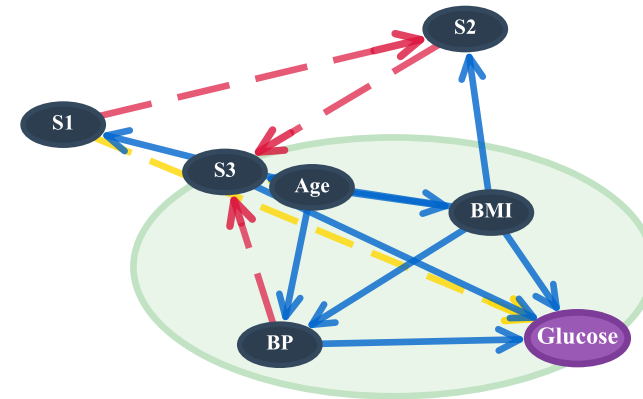
50% missing, F1=0.78
