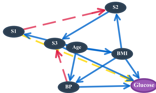
30% missing, F1=0.84
