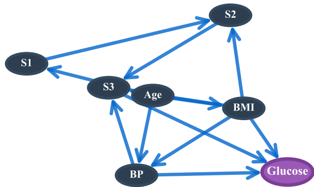
0% missing, F1=1.00
