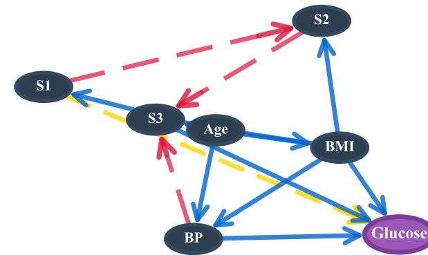
50% missing, F1=0.78
