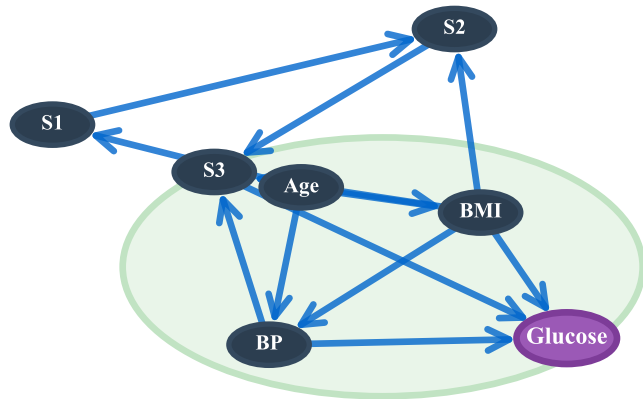
0% missing, F1=0.93
