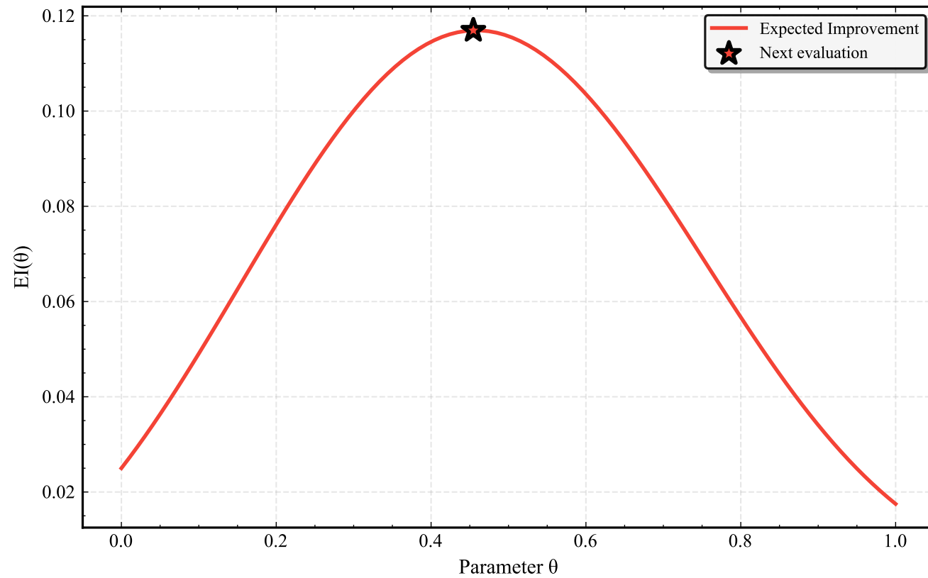
(c) Expected Improvement Acquisition
