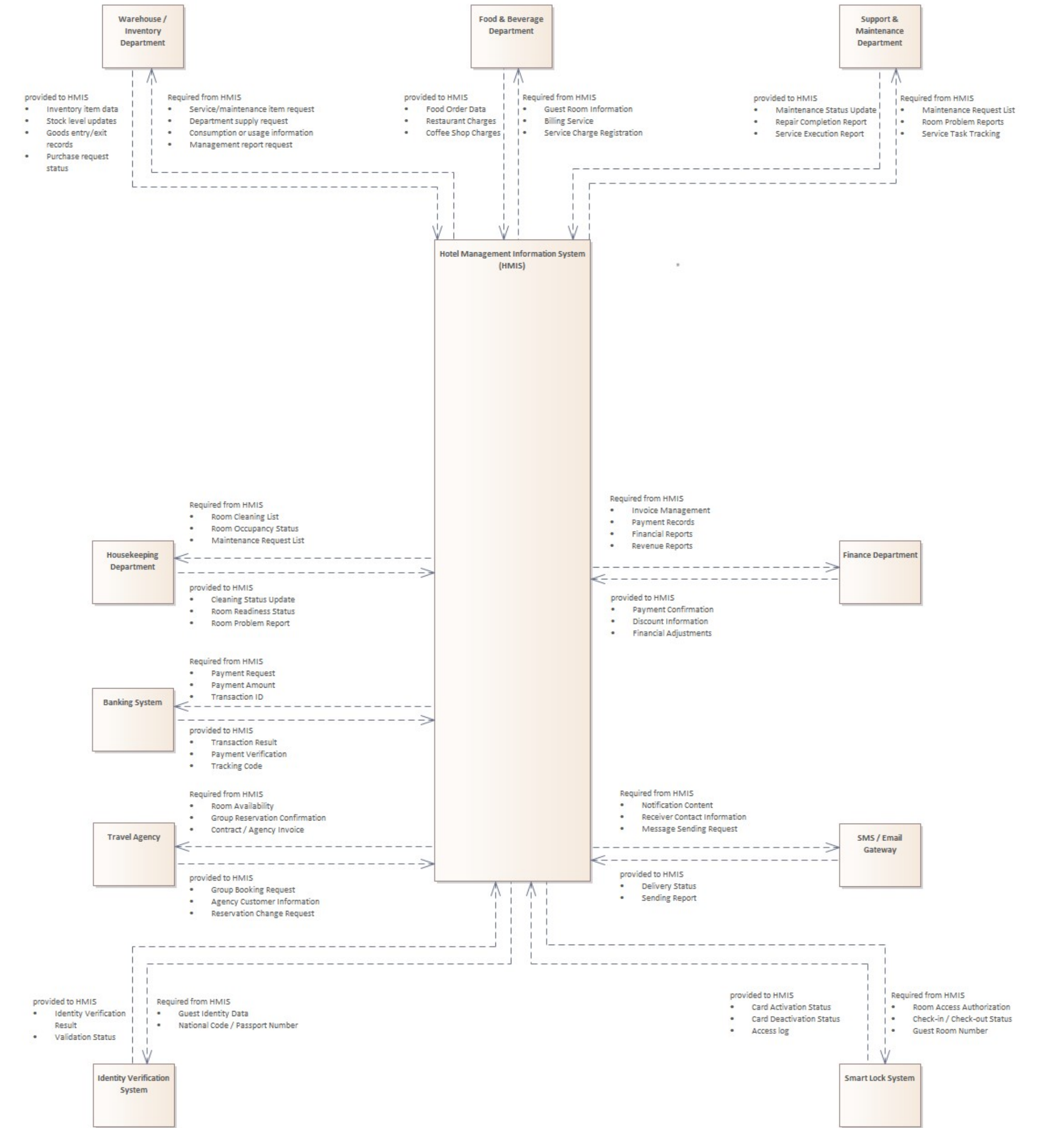
class Context Diagram - HMIS
