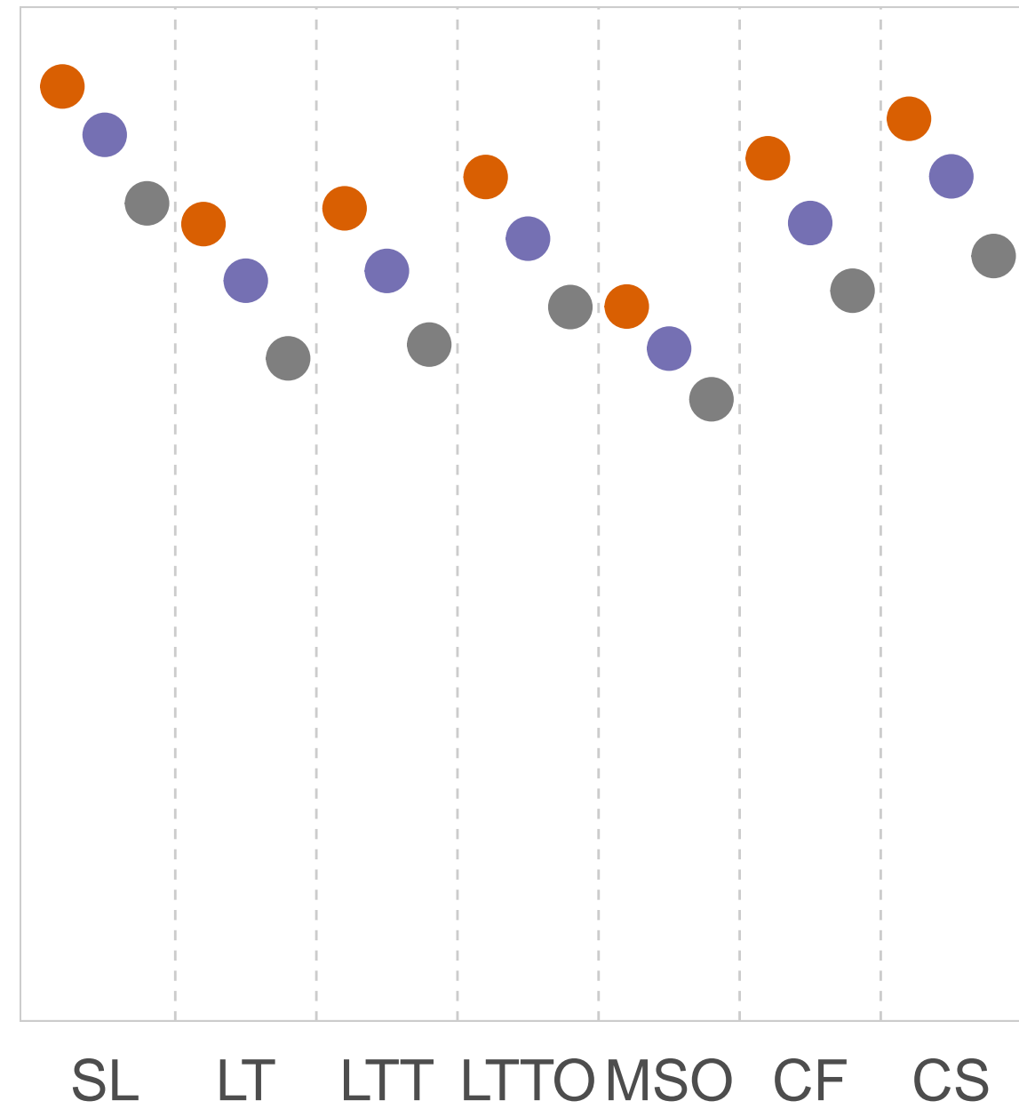
RNN
