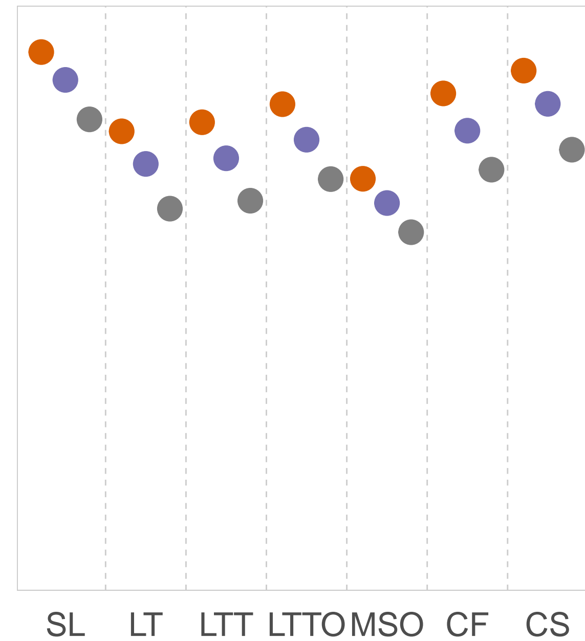
RNN
