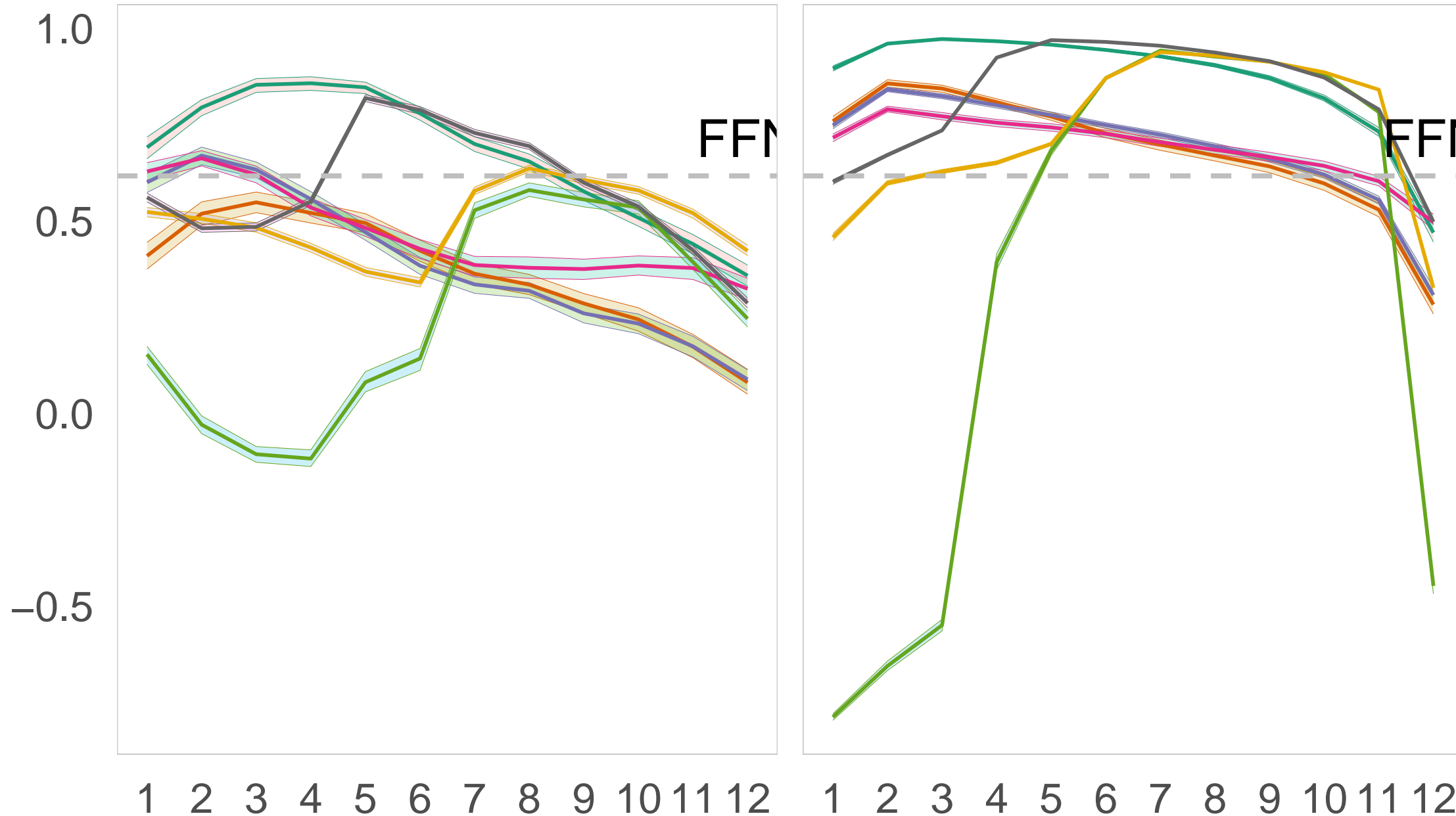
Brier Skill Score
