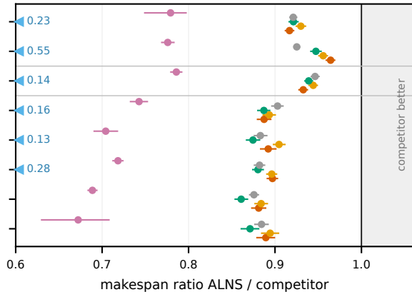
(b) C1: ALNS on 8 cores at B_1
