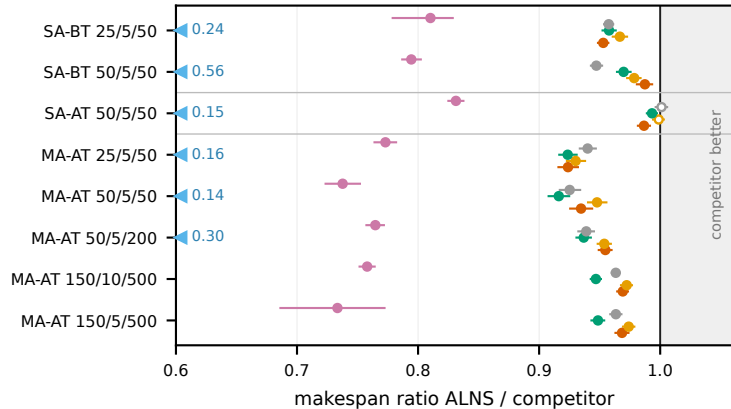
(a) C2: ALNS on 1 core for 2 s
