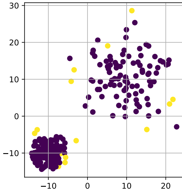
LOF Model
