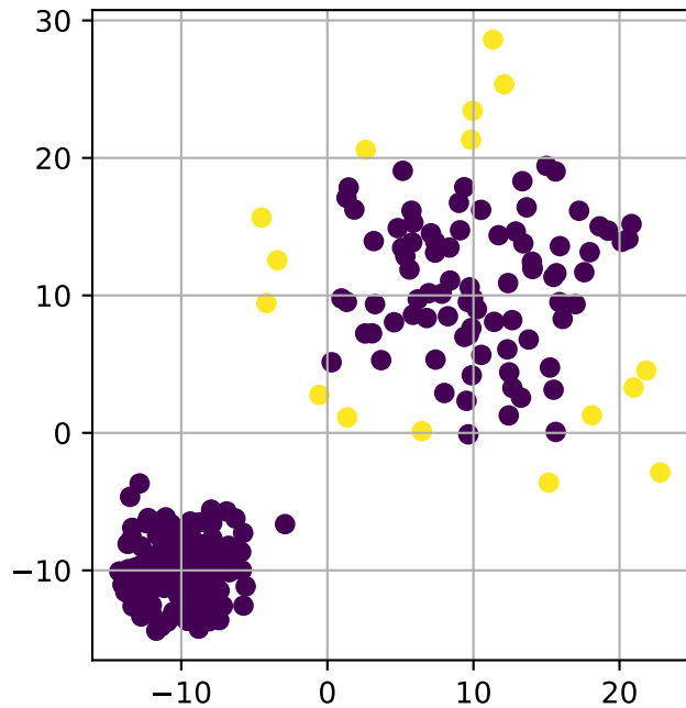
KNN Model
