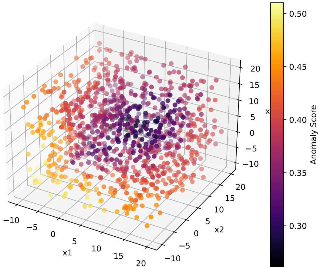
DIF 3D Anomaly Scores
