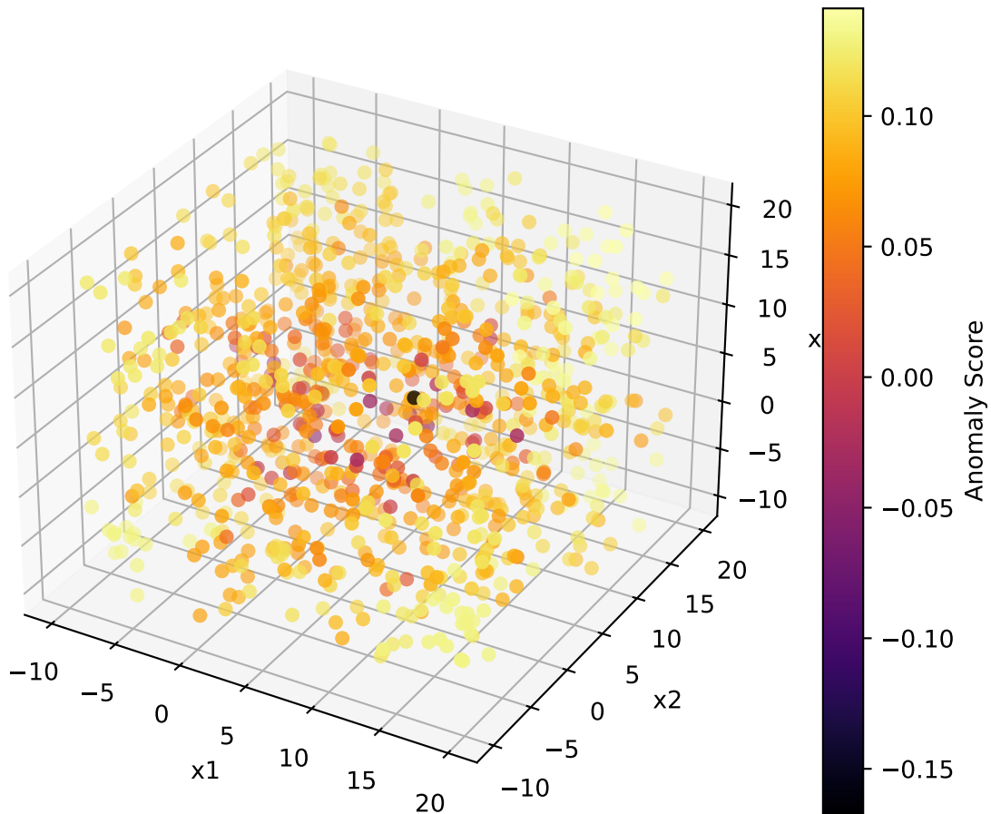
IForest 3D Anomaly Scores
