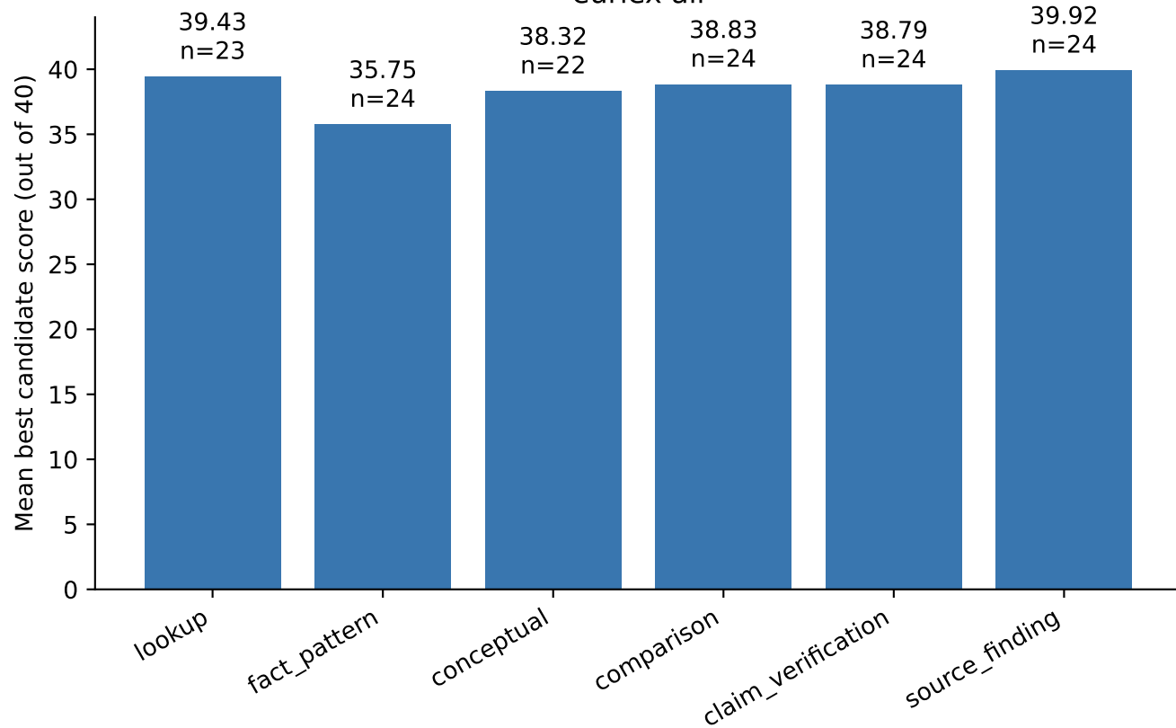
eurlex all
