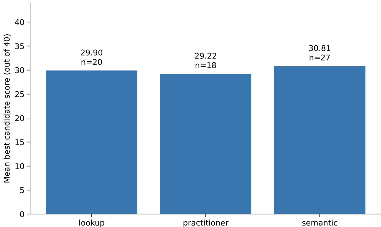
Mode comparison: non-meeting targets with a scored candidate
