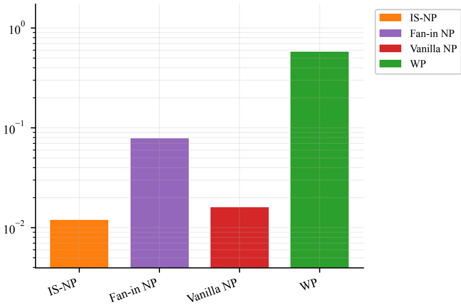
Estimator variance (log scale)
