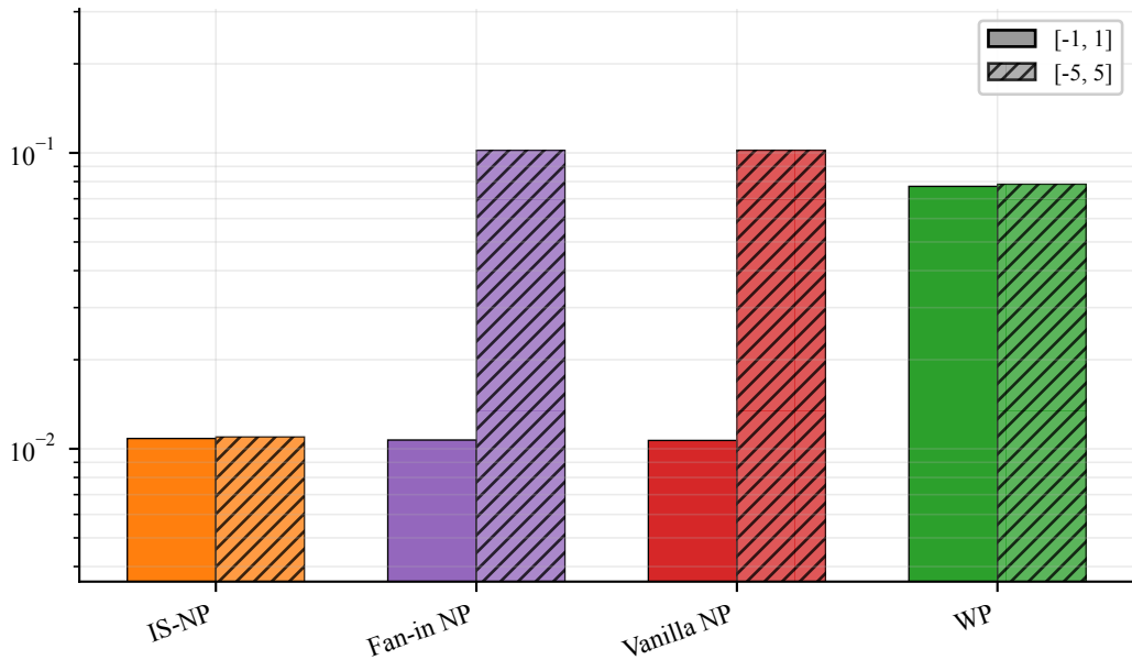
Estimator variance (log scale)
