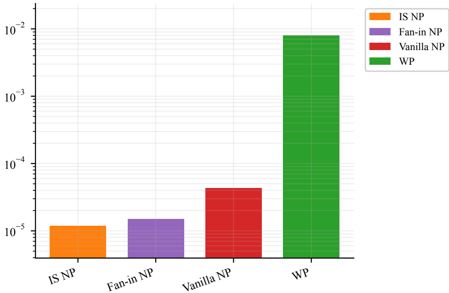
Update variance (log scale)
