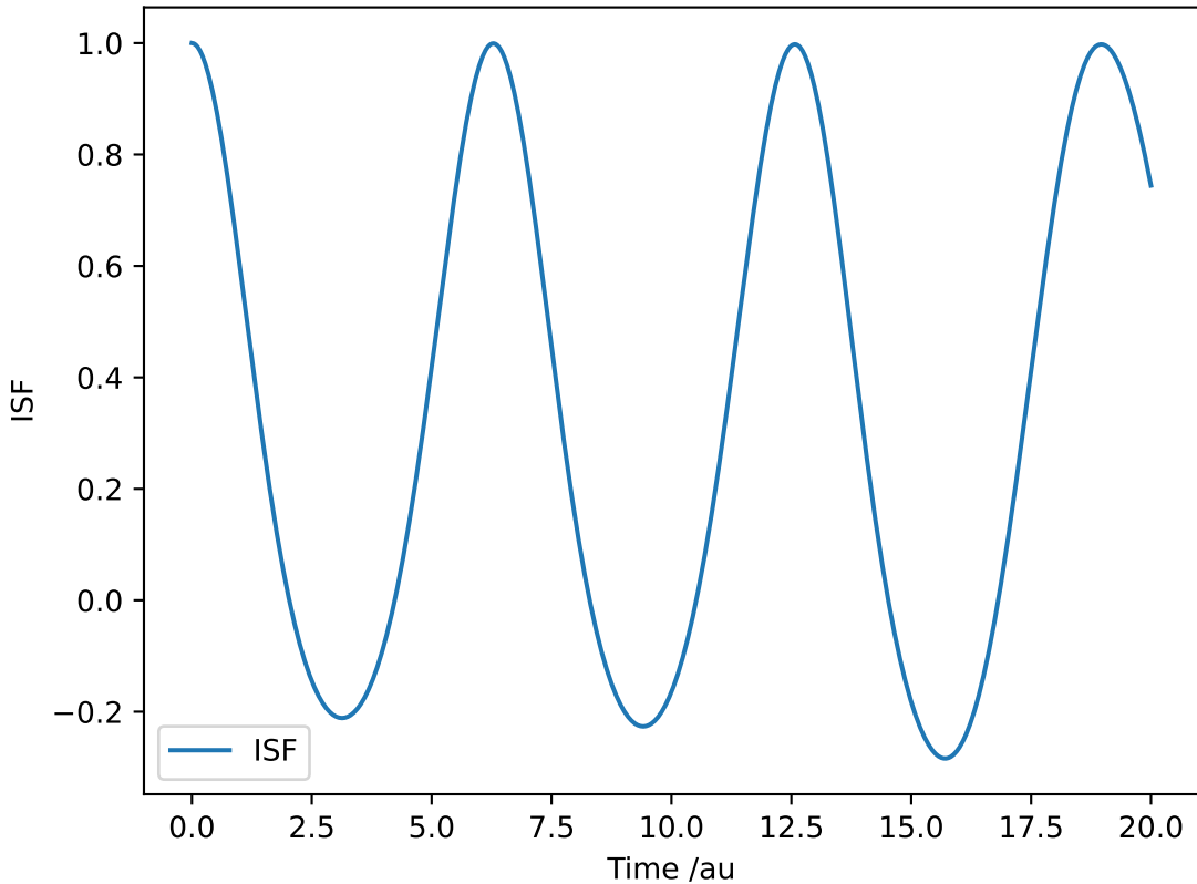
Intermediate Scattering Function Over Time
