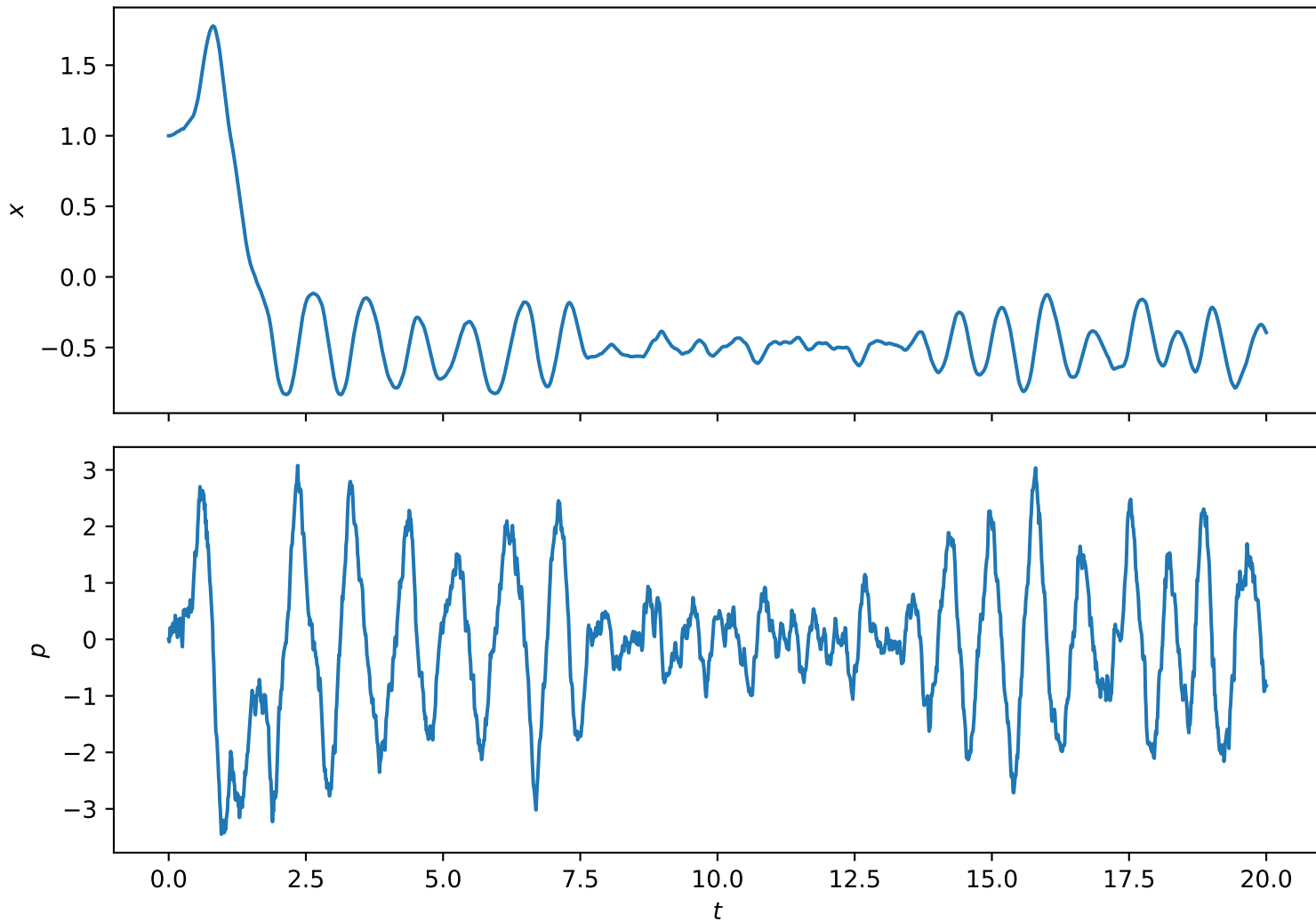
Position and Momentum Evolution
