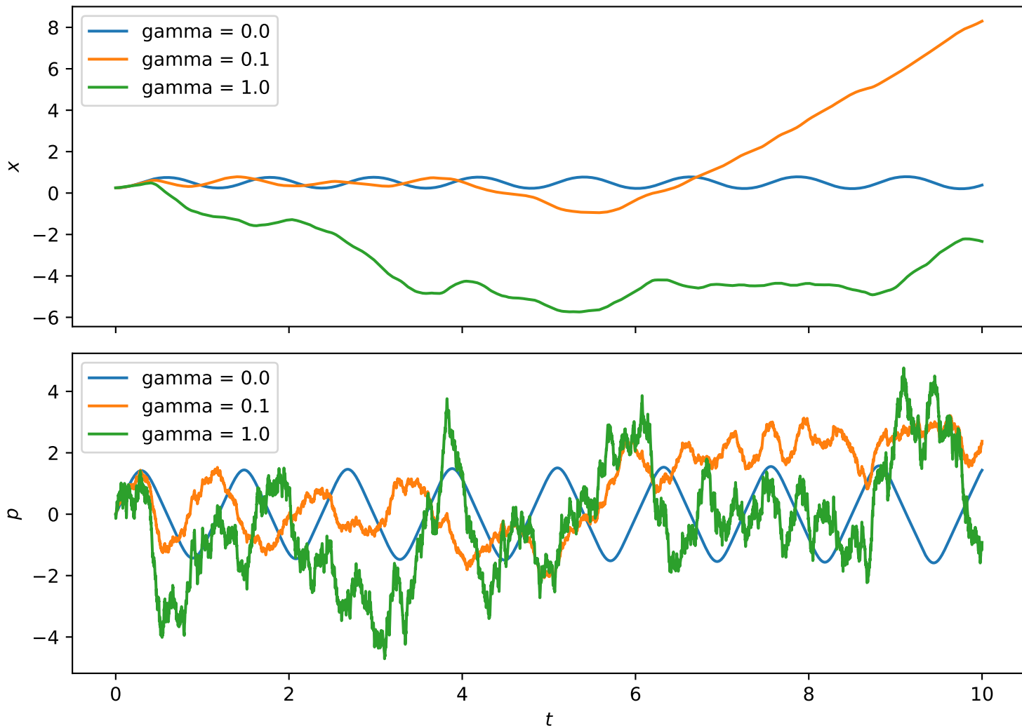
Position and Momentum Evolution
