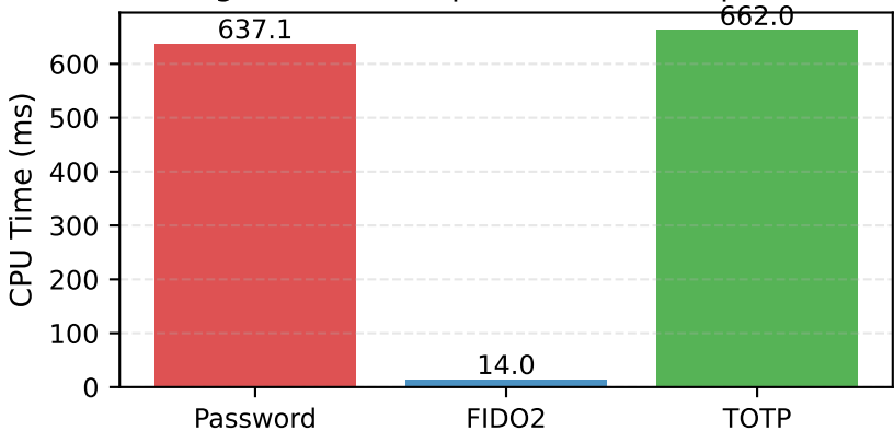
Registration/Setup CPU Time Comparison
