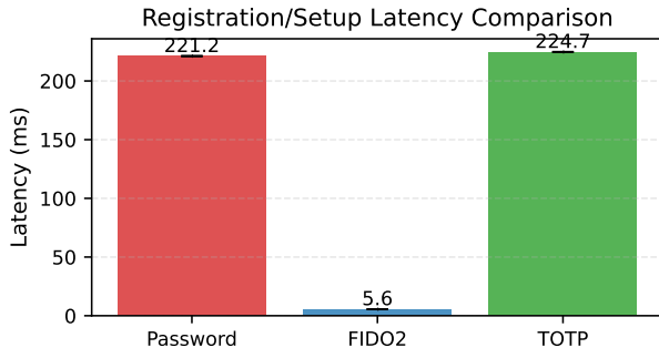
Fig. 4. Registration latency comparison between Password and FIDO2 authentication methods. Error bars show min-max range.
