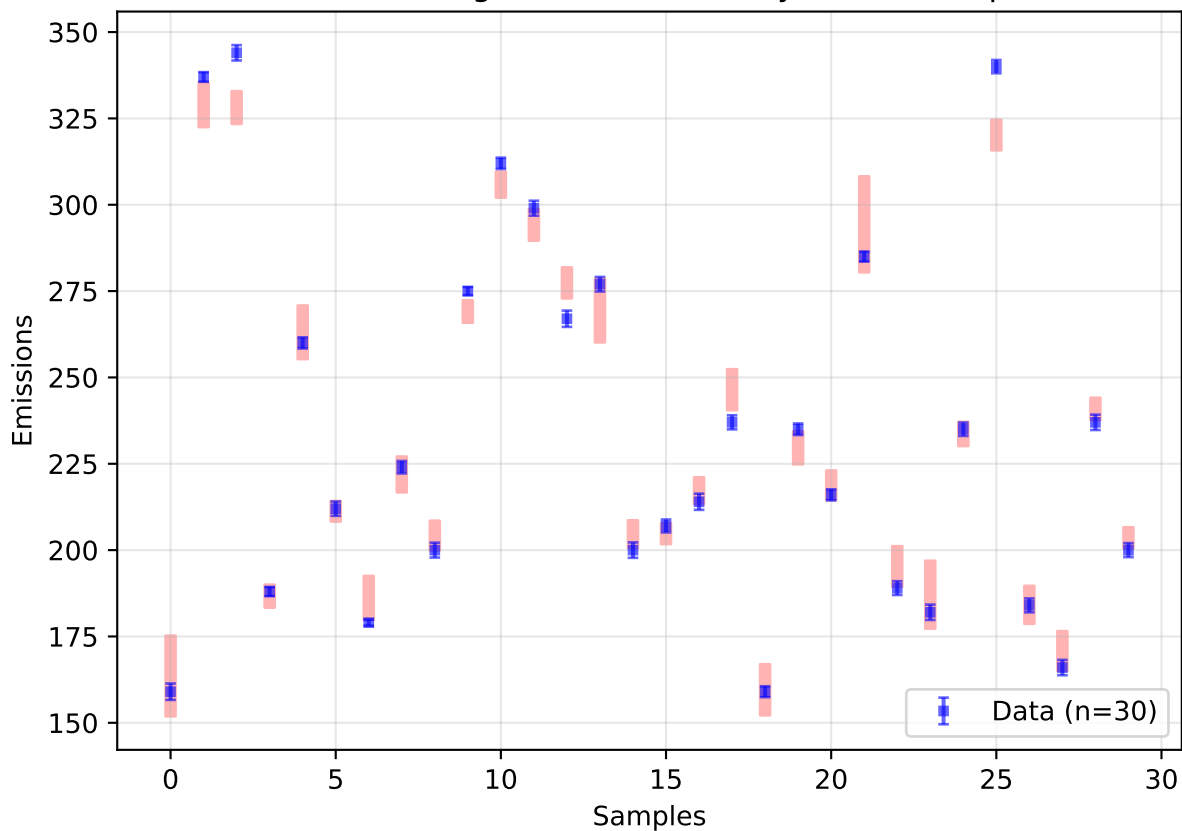
Multivariate Regression with Chebyshev Basis ( p=3 )
