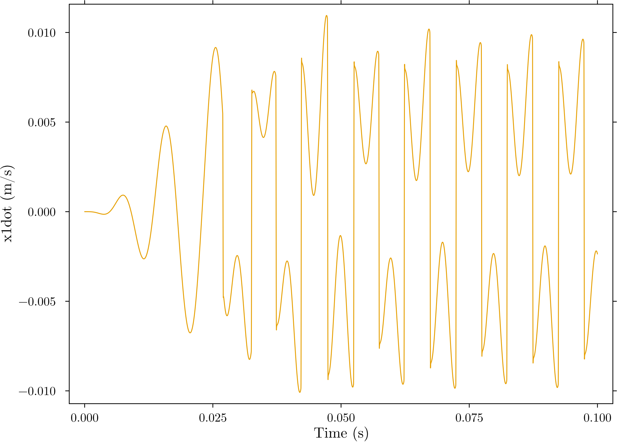
Shuttle Mass Velocity (x1dot)
