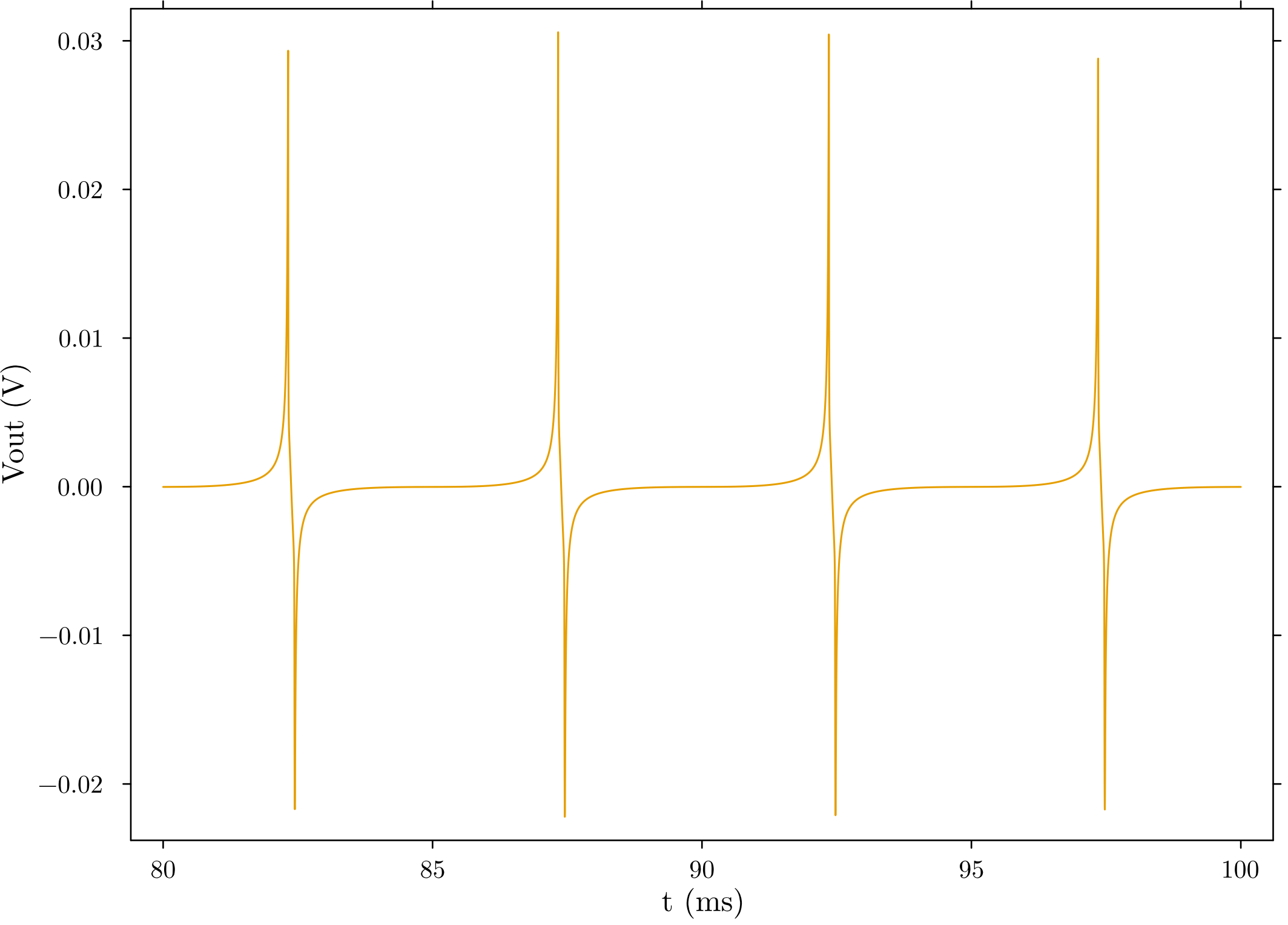
Output Voltage (state) - last 2 cycles
