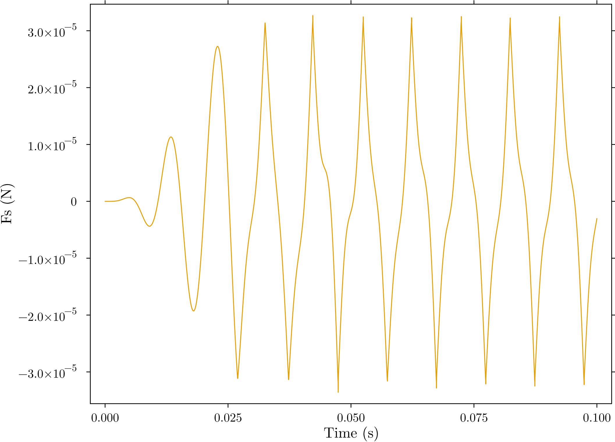
Suspension + Stopper Force on x1 (incl. -c_1 \cdot \dot{x}_1 )
